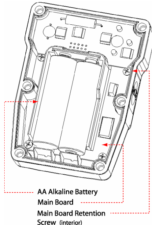
Figure 5.1: Interior view
